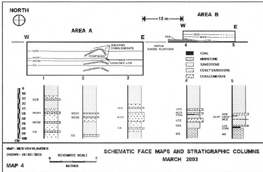
Map 4 – Schematic face maps and stratigraphic columns
